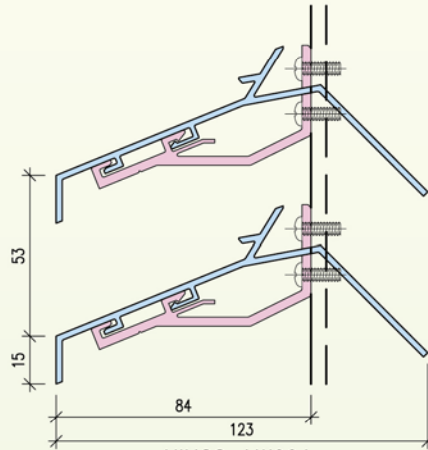
HINGSS-LW601 FREE AREA = 65.5% WATER PENETRATION CLASS = B ~ C DISCHARGE LOSS COEFFICIENT CLASS = 2
