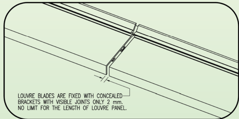
HINGSS-LW901 FREE AREA = 60.5% WATER PENETRATION CLASS = C ~ D DISCHARGE LOSS COEFFICIENT CLASS = 2
